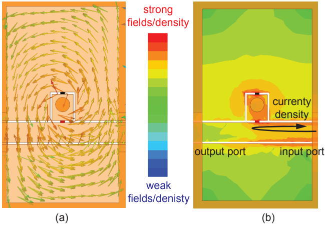
Fig. 2. HFSS simulation of a single bandstop resonator at resonant frequency. Results show the (a) magnetic fields excited in the substrate and (b) the current density flows from the input port into the resonator.
