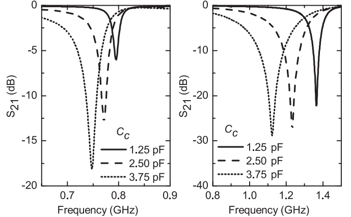
Fig. 3. Simulation from HFSS shows tunable bandwidth at the (a) lower tunable frequency and at the (b) higher tunable frequency.
