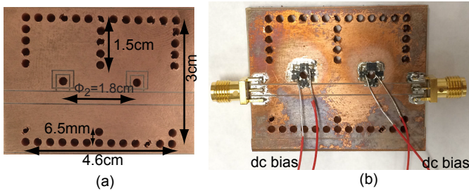
Fig. 4. Fabricated two-pole band stop filter (a) without the surface mount diodes and (b) with the surface mount diodes.
