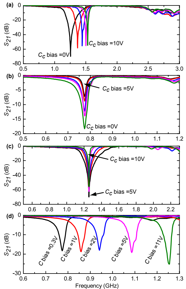
Fig. 5. Measured s-parameters of fabricated filter where (a) shows tunable bandwidth, (b) and (c) show tunable bandwidth at a fixed frequency and (d) shows a constant 83 MHz bandwidth across the tuning range.
