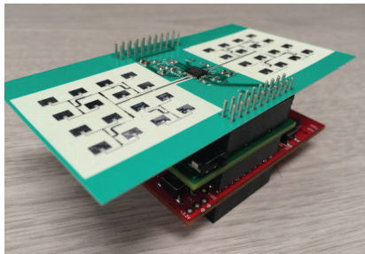
24 GHz radar module with array antenna and embedded processing
